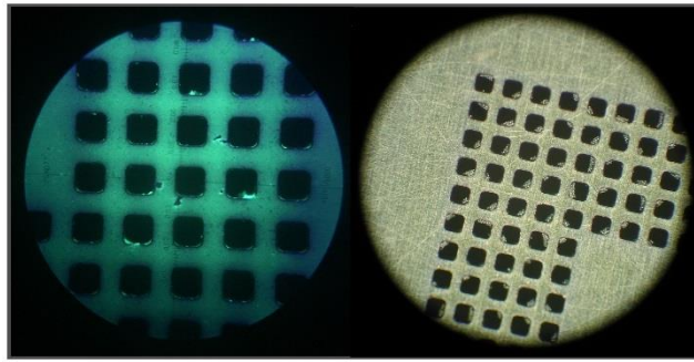
Figure 12: FPN Coating, 1000 Dry Wipes (left), 20 Prints with No Underside Wipe
